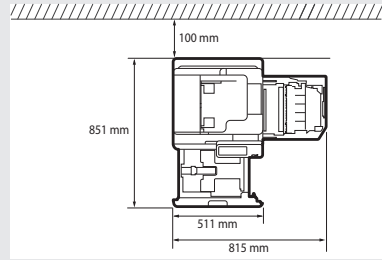
imageRUNNER C1335iF
