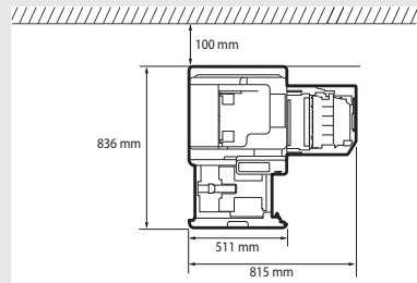
imageRUNNER C1325iF
