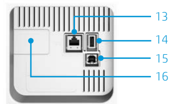
Rear I/O panel close-up
