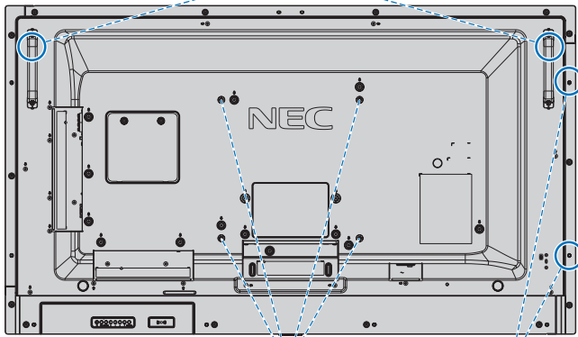
VESA Mounting Interface (M6)
