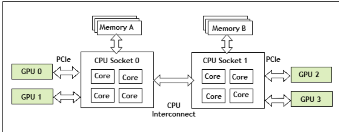
Figure 34 A NUMA server platform
