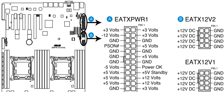
Z9PR-D12/4L ATX power connectors
