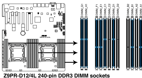
Z9PR-D12/4L 240-pin DDR3 DIMM sockets
